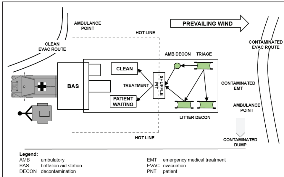
Figure 5-3. Battalion aid station using the chemical-biological protective shelter
