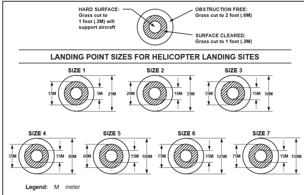
Figure C-1. Landing point sizes
