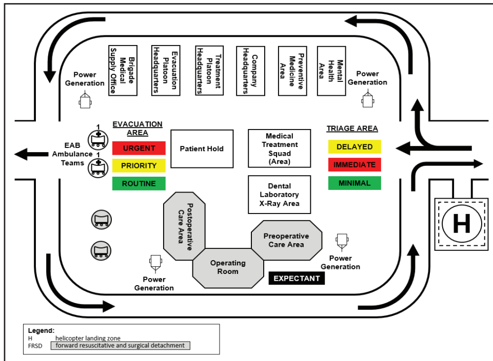
Figure 1-21. Example, brigade support medical company with attached forward resuscitative and surgical detachment layout
